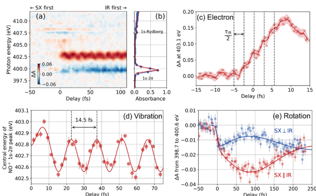
Fig. 2. (a) Time-resolved absorption spectra of NO. (b) Static absorbance of NO without the pump pulses measured in our experiment (blue circles) and a synchrotron (red curve). (c) Absorbance change of the NO + 1s\text{-}2\pi peak at 403.1 eV (red circles) and its 3-point rolling average (red curve). (d) Central energy of the NO + 1s\text{-}2\pi peak (red circles) and the fitting by a cosine and Gaussian function (red curve). (e) Absorbance change of the NO 1s\text{-}2\pi peak (398.7 to 400.6 eV) with parallel (red circles) and perpendicular (blue circles) IR and SX polarizations. The solid curves are calculation results considering molecular alignment. The pump intensity is \sim 1 \times 10^{14} \text{ W/cm}^2 for (a, b, d, e) and \sim 2 \times 10^{14} \text{ W/cm}^2 for (c). The polarizations of the IR and SX are parallel for (a, c, d).
