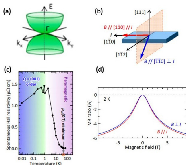
Fig. 1. (a) Band structure of a Luttinger semimetal consisting of quadratic band touching of 5d electrons at the \Gamma point near E_F (b) Schematic for experimental configurations of magnetotransport measurements. (c) Temperature dependence of the spontaneous Hall resistivity. (d) Magnetoresistance curves as a function of the magnetic field B measured at 2 K for B \parallel I and B \perp I configurations. The solid and dotted lines are up and down sweeps of B , respectively. The difference between the two curves arises from the chiral anomaly and indicates that the film is in the Weyl semimetal state.
