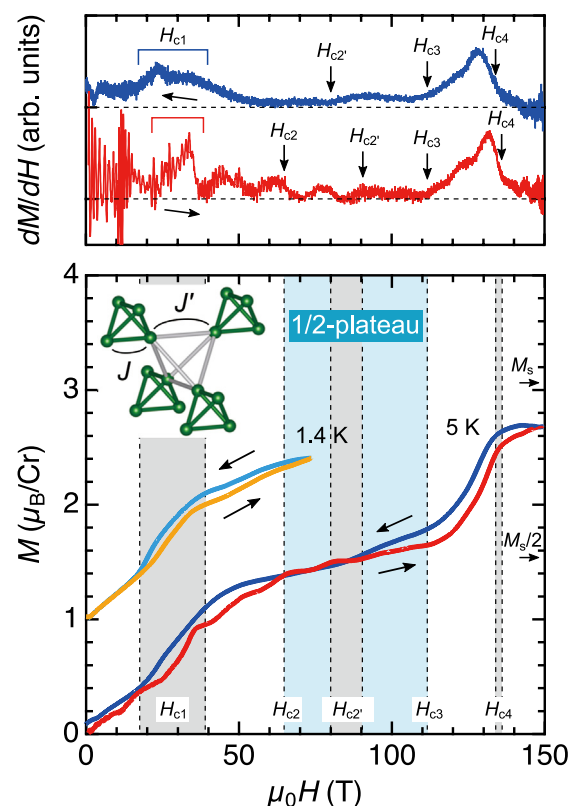
Fig. 1. M - H curves of CuInCr 4 S 8 measured at \sim 5 K in a single-turn coil megagauss generator up to 150 T (red and blue curves for up and down sweeps, respectively). Derivatives dM/dH are shown in the upper panel. The previously reported M - H curve measured at 1.4 K up to 73 T are also shown (orange and cyan curves for up and down sweeps, respectively) [3]. Transition fields are denoted by brackets or arrows in the upper panel, and drawn by the shaded areas (first order) or dashed lines (second order) in the lower panel. Inset shows the schematic of the breathing pyrochlore lattice.
