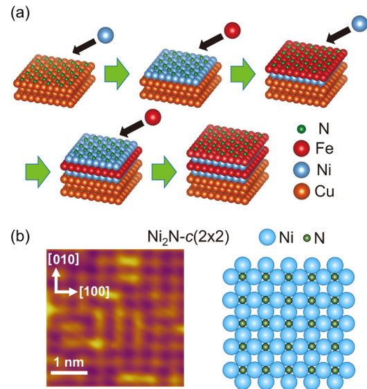
Fig. 1. (a) Schematic model of an FeN/Ni/Fe/Ni film formation process on Cu(001) by surfactant epitaxy using N atoms. First, monolayer c(2 \times 2) \text{Ni}_2\text{N} is formed on Cu(001) surface as shown in (b) by N adsorption and Ni deposition. Then, 1-ML Fe is deposited below 150 K. After annealing above 300 K, N atoms segregate to the Fe surface and \text{Fe}_2\text{N} monolayer is formed. Next, on top of this surface, 1-ML Ni is deposited below 150 K. By repeating deposition and annealing, the L1_0 FeNi film is prepared. (b) STM image of a \text{Ni}_2\text{N} atomic layer on Cu(001) (left) and its ball model (right). The 0.5-ML N form c(2 \times 2) structure with 1 \times 1 Ni atoms [1].
