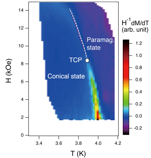
Fig. 2. Phase boundary between the paramagnetic and the single- q helical (conical) states of EuPtSi, constructed by colour contour mapping of the dM/dT data with H \parallel [110] . The bright line in low fields indicates the first-order boundary, whereas the dashed line shows the second-order one. TCP denotes the position of the tricritical point.
