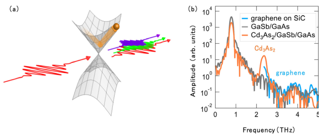
Fig. 1. (a) A schematic of high harmonic generation due to the coherent acceleration of Dirac electrons. (b) Amplitude spectra of the transmitted intense THz pulse with appearance of the THz THG in \text{Cd}_3\text{As}_2 thin film.
