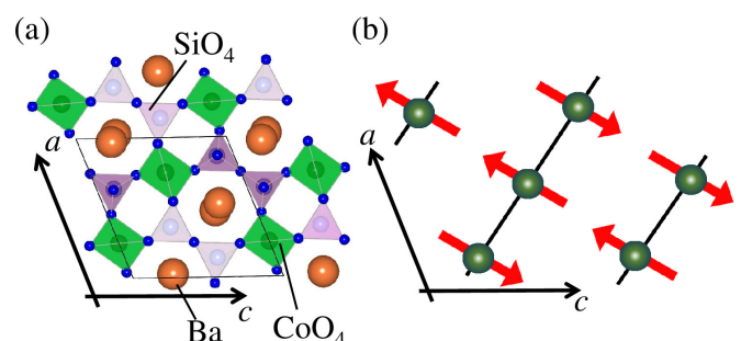
Fig. 1. (a) Crystal structure of Ba 2 CoSi 2 O 7 . (b) Schematic magnetic structure of Ba 2 CoSi 2 O 7 .
