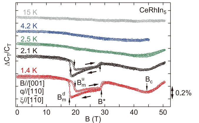
Fig. 1. Magnetic field dependence of the transverse elastic constant \Delta C_T/C_T at several temperatures for B//[001] . The vertical arrows indicate the metamagnetic transition field B_m^{u(d)} for field up(down) sweep, the EN transition field B^* , and the critical field B_c . The right and left arrows show hysteresis direction. The propagation direction q and polarization direction \xi of ultrasound are indicated.
