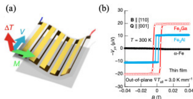
Fig. 1. (a) Thermopiles based on the ANE. V , M , and \Delta T is the voltage, magnetization, and temperature difference, respectively. (b) Magnetic field dependence of the Nernst voltage -V_N for the thin films of Fe 3 Ga, Fe 3 Al and \alpha -Fe. The temperature gradient in the sample (MgO substrate/Fe 3 Ga, Fe 3 Al, or \alpha -Fe/MgO), \nabla T_{\text{all}} , is monitored to be 3.0 \text{Kmm}^{-1} . The temperature gradient in the Fe 3 Ga (Fe 3 Al) layer is estimated to be \nabla T \approx 0.86 \text{Kmm}^{-1} (1.0 \text{Kmm}^{-1} ).
