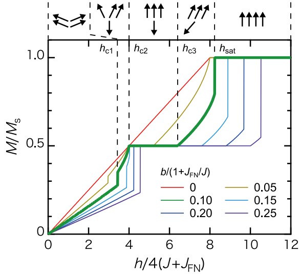
Fig. 2. Calculated magnetization curves as a function of magnetic field h for b/(1 + J_{\text{FN}}/J) = 0 to 0.25 in steps of 0.05. The spin structures corresponding to the curve for b/(1 + J_{\text{FN}}/J) = 0.10 (thick green line) are shown in the upper part of the figure.
