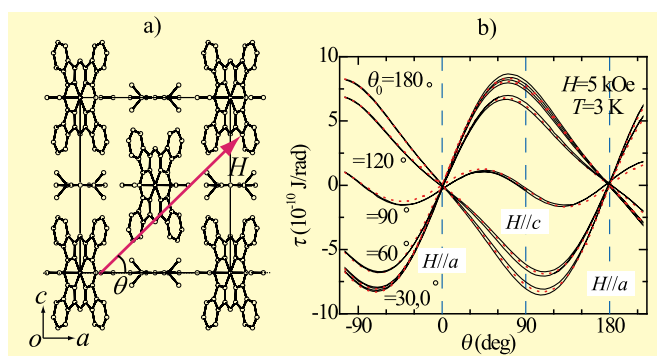
Fig. 1. (a) The definition of the field direction and crystal structure of PTMA 0.5 [Fe(Pc)(CN) 2 ] \cdot CH 3 CN. (b) Magnetic torque curves at 3 K for the field of 0.5 T rotated within the ac -lane. In this measurement, the magnetic field of 40 kOe was applied at 10 K along the direction of \theta = \theta_0 , and the sample was cooled down to 3 K in the same field. Torque curves were measured in the reduced field of 5 kOe. Black solid lines illustrate the observed data of torque curves, while the red dotted lines are the fit of Eq. (1) to the solid lines.
