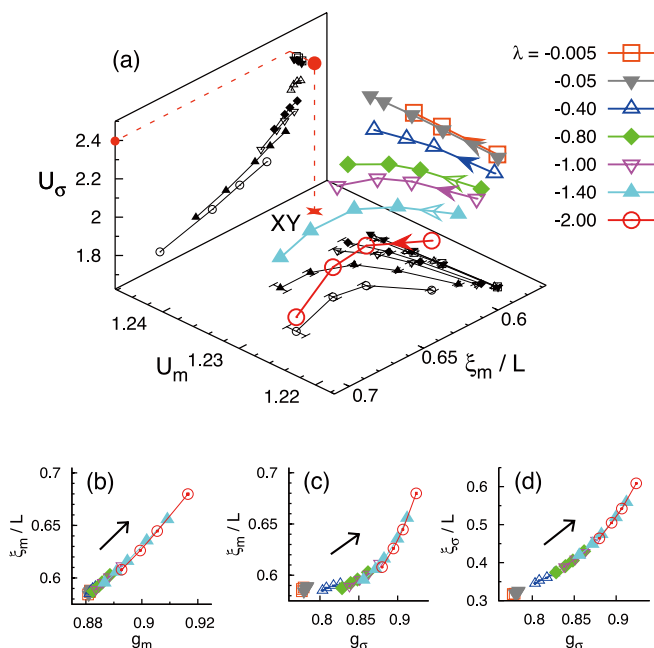
Fig. 3. The flow diagram of dimensionless scaling parameters (6 parameters in total). (a) A three-dimensional (3D) projection onto ( U_m , \xi_m/L , U_\sigma ) space and (b–d) two-dimensional projections are shown. Because of the approximately single curve found in a four-parameter subspace ( g_m , \xi_m/L , g_\sigma , \xi_\sigma/L ), the analysis of the flow structure can be reduced to the 3D flow diagram. The arrows show directions of the flow lines. The estimated location of the unstable XY fixed point ( U_m , \xi_m/L , U_\sigma ) = (1.2430(5), 0.5925(2), 2.40(1)) is indicated by a large filled circle. See Ref. [2] for further details.
