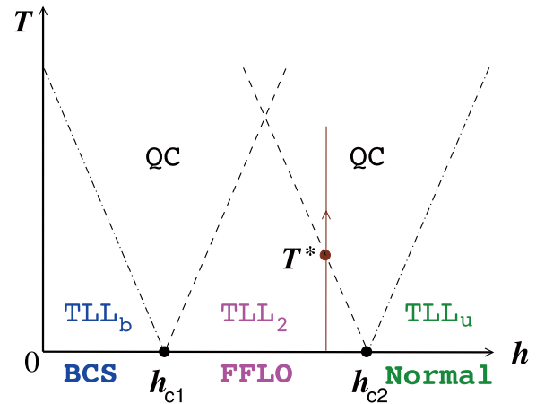
Fig. 2. (From Ref. [1]) Schematic finite-temperature "Phase diagram". The three phases at zero temperature correspond to distinct Tomonaga-Luttinger liquid phases. The crossover lines, which emerge from the quantum phase transition points, represent breakdown of the Tomonaga-Luttinger liquid theory.
