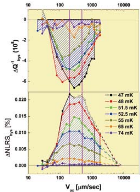
Fig. 1. "hysteretic" \Delta\text{NLRS}_{\text{hys}} = \text{NCRI}F as well as \Delta Q_{\text{hys}}^{-1} vs \log V_{ac} . The hysteretic behavior starts at V_{ac} \geq 40 \mu\text{m/s} at all T 's below \sim 75 \text{ mK} . And both \Delta\text{NLRS}_{\text{hys}} and \Delta Q_{\text{hys}}^{-1} reach some extreme values for the range V_{ac} = 200 - 500 \mu\text{m/s} . Then the absolute size of both quantities starts to decrease. We observe nearly \log V_{ac} linear decreases especially for \Delta\text{NLRS}_{\text{hys}} . From this linear extension of the \log V_{ac} dependence we obtain a critical velocity, 6\text{--}10 \text{ mm/s} to suppress the \text{NCRI}F = \rho_{ss} to zero, which compares well with V_c = \hbar/(m^4 \xi_0 \pi) = \sim 6\text{--}12 \text{ mm/s} , for \xi_0 = 50\text{--}25 \text{ nm} . See text.
