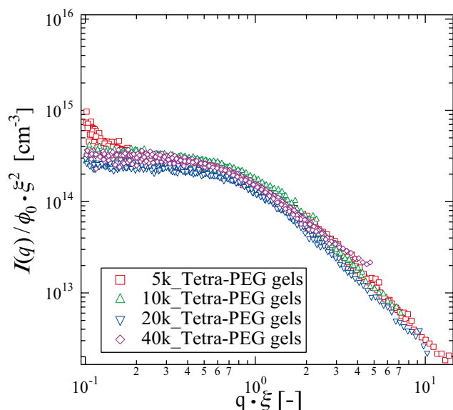
Fig. 2. SANS master curves for as-prepared Tetra-PEG gels ( M_w = 5, 10, 20 , and 40 kg/mol). All SANS curves can be superimposed to a single master curve by using the reduced variables of \xi q and I(q)/\phi_0 \xi^2 .
