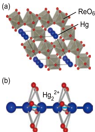
Fig. 1. (a) Crystal structure of the hexagonal bronze \text{Hg}_{2/3}\text{ReO}_3 , which is composed of corner-shared \text{ReO}_6 octahedra and Hg polycations in the open tunnels. The solid line shows a primitive unit cell. (b) Coordination environment of an \text{Hg}_2^{2+} polycation.
