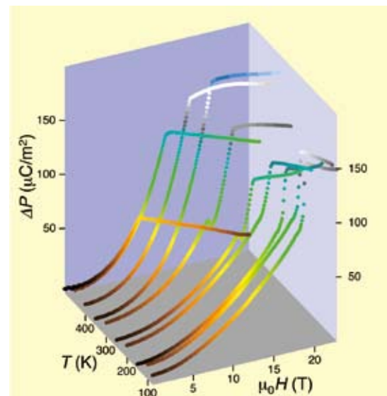
Fig. 2. Magnetic field-induced changes in P ( \Delta P ) projected to the cubic [001] direction at various temperatures from 77 K to 500 K. Magnetic fields were applied perpendicular to the projection axis. The transition field becomes smaller with increasing the temperature toward the Néel temperature of \sim 600 \text{ K} . The field-induced change in P remains larger than 100 \mu\text{C}/\text{m}^2 up to 450 K.
