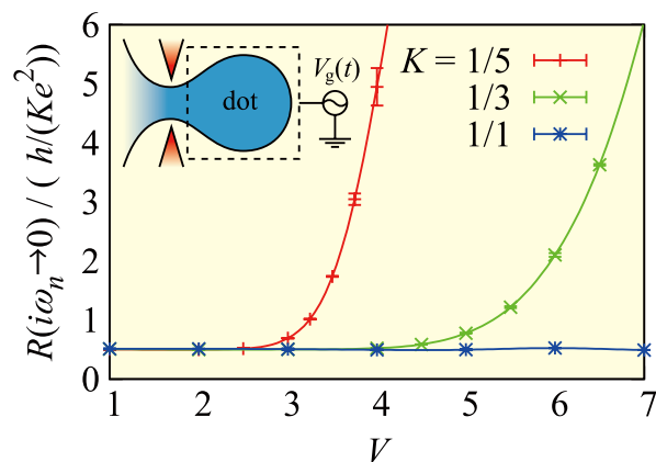
Fig. 1. Dynamic resistance as a function of reflection strength V at QPC. For K=1 , it remains constant, while for K<1 it rapidly increases beyond a critical value of V . Inset, a schematic picture of the mesoscopic capacitor.
