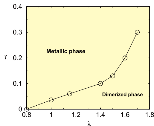
Fig. 1. Phase diagram of the one-dimensional spinful Holstein model with anharmonicity in the (\lambda, \gamma) -plane where \lambda is an electron-phonon coupling constant and \lambda is the coefficient of the quartic term of the potential.
