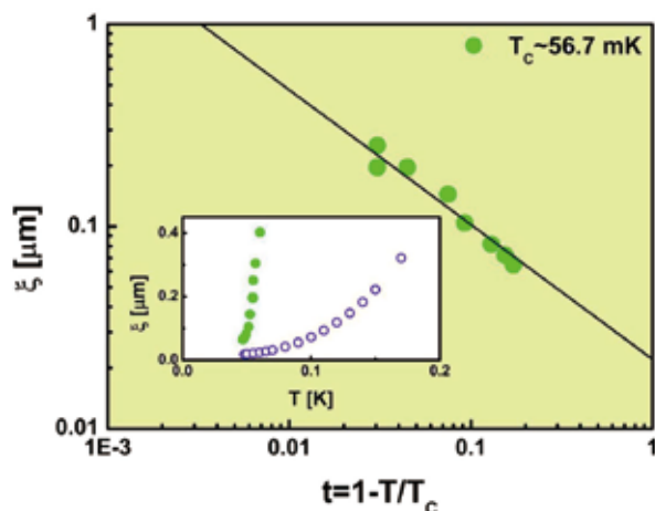
Fig. 2. Critical behavior of \xi obtained from the T dependent \Delta NLRS_{\text{hys}} = \rho_{ss} data at 200 \mu\text{m/s} in Fig. 1. We took T_c = 56.7 mK, supposing \rho_{ss} = (1 - T/T_c)^\gamma with \gamma = 2/3 . We obtain \xi_0 \sim 25 to 50 nm by simple extrapolations, horizontal and straight extension of the linear relation. Inset shows \xi for the SS state \xi_{SS} as well as for the VF state \xi_{VF} in linear scales. \xi_{SS} > \xi_{VF} at all T where they coexist.
