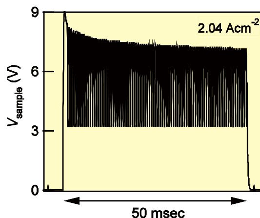
Fig. 2. V_{\text{sample}} oscillation under applied dc current 1.86 \text{A cm}^{-2} at 230 K for \beta -(BEDT-TTF) _2 PF _6 .
