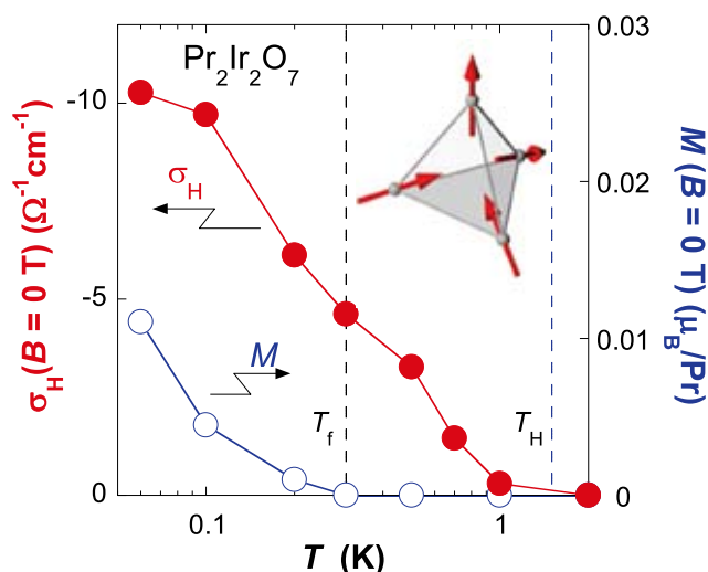
Fig. 1. Temperature dependence of the remnant Hall conductivity \sigma_H(B=0) (left axis) and remnant magnetization M(B=0) (right axis) at zero field, obtained after a field sweep down from 7 T in the hysteresis loop measurements of the pyrochlore oxide \text{Pr}_2\text{Ir}_2\text{O}_7 . Inset: unit of the pyrochlore lattice “2-in, 2-out” configuration of four \langle 111 \rangle Ising spins on a tetrahedron.
