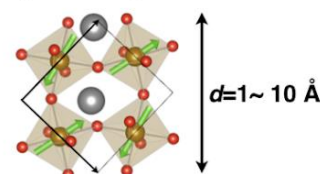
Phonons / Magnons E = 1 \sim 100 \text{ meV}
