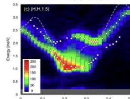
Phonons / Magnons E = 1 \sim 100 \text{ meV}
