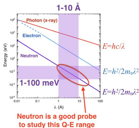
Crystal / Magnetic structure
